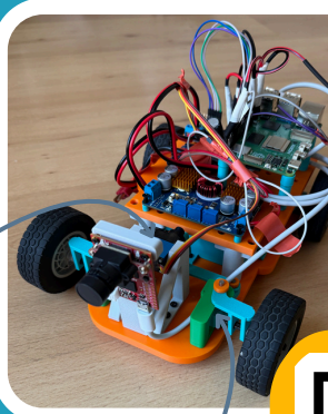
Steering gear
